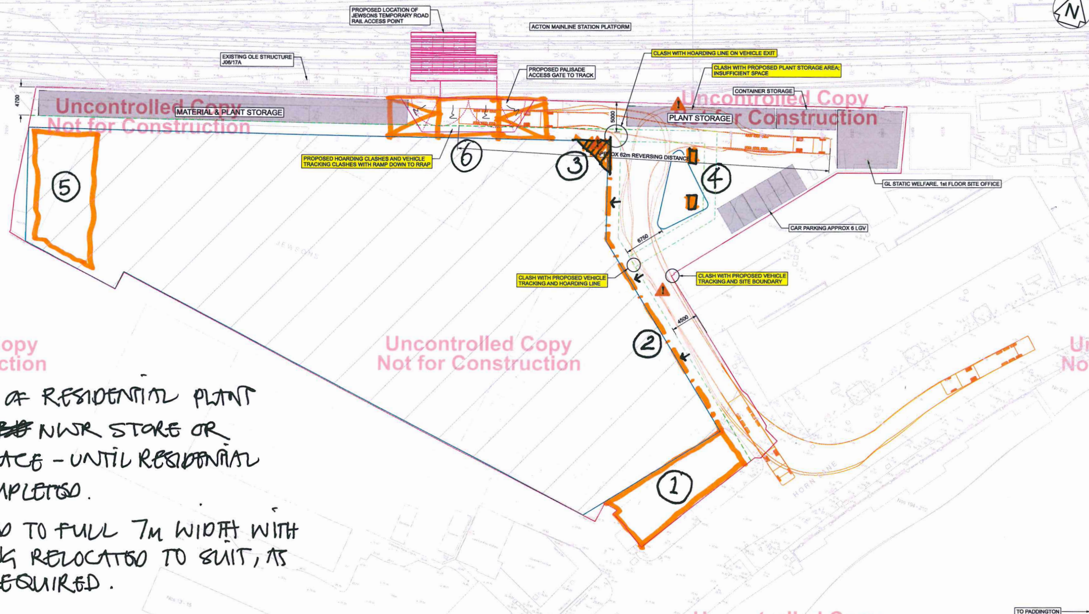
2 JEWSON'S YARD - SITE LAYOUT GENERAL ARRANGEMENT 136002 SCALE 1:250
