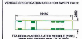
1 DETAIL 1 136002 SCALE 1:250
