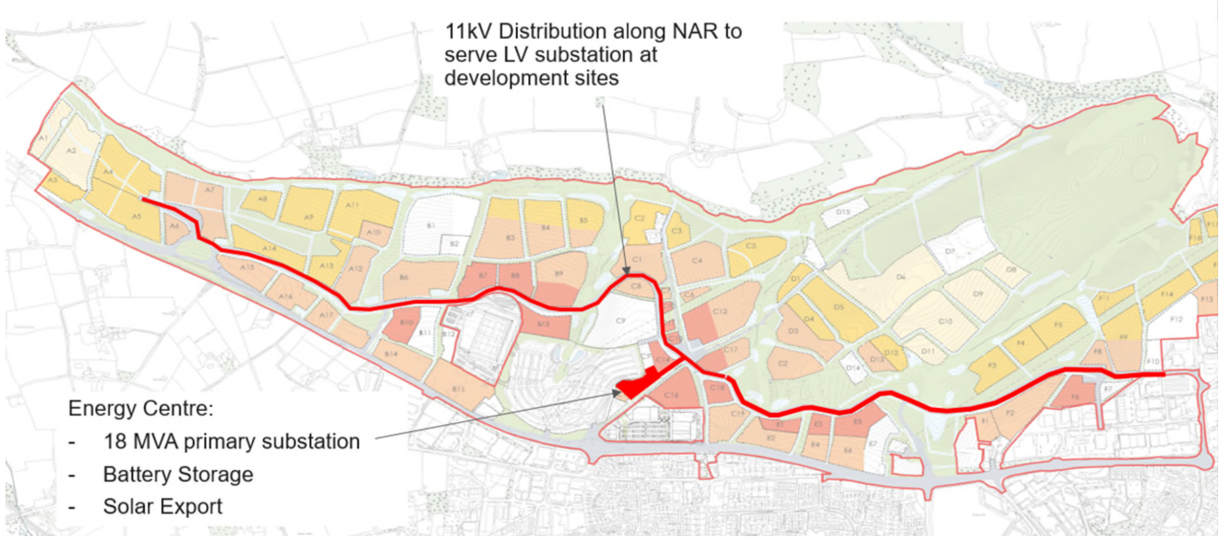
Figure 14 - Proposed Strategic Power Infrastructure
