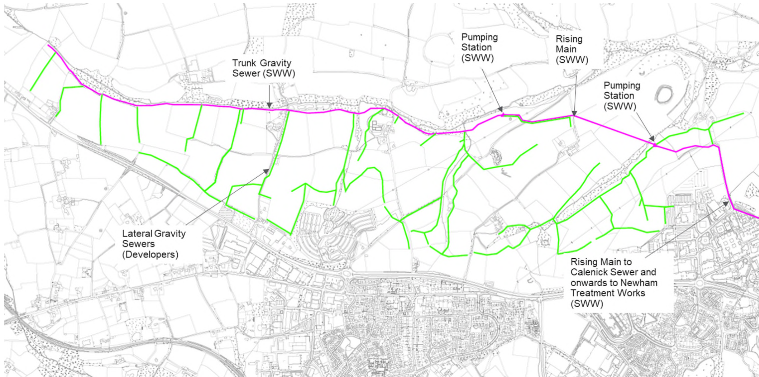
Figure 9 – Strategic Foul Sewer Infrastructure
