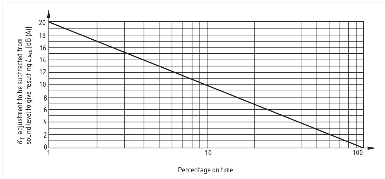
Figure F.5 Adjustment to sound level to give resulting L_{Aeq} (plant sound power method)
