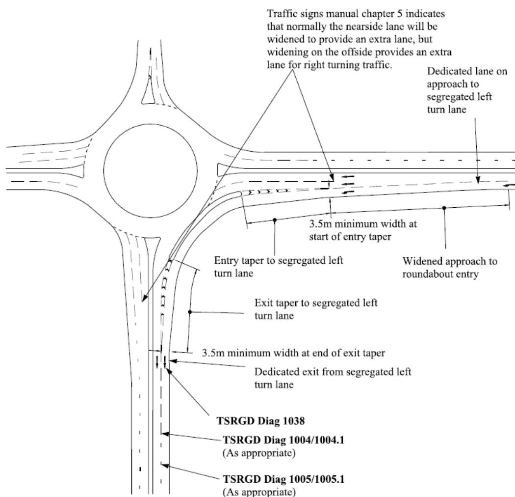
Figure 6.27N2a Dedicated approach and exit for SLTL
