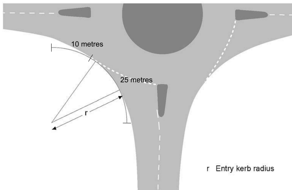
Figure 3.19 Entry kerb radius
