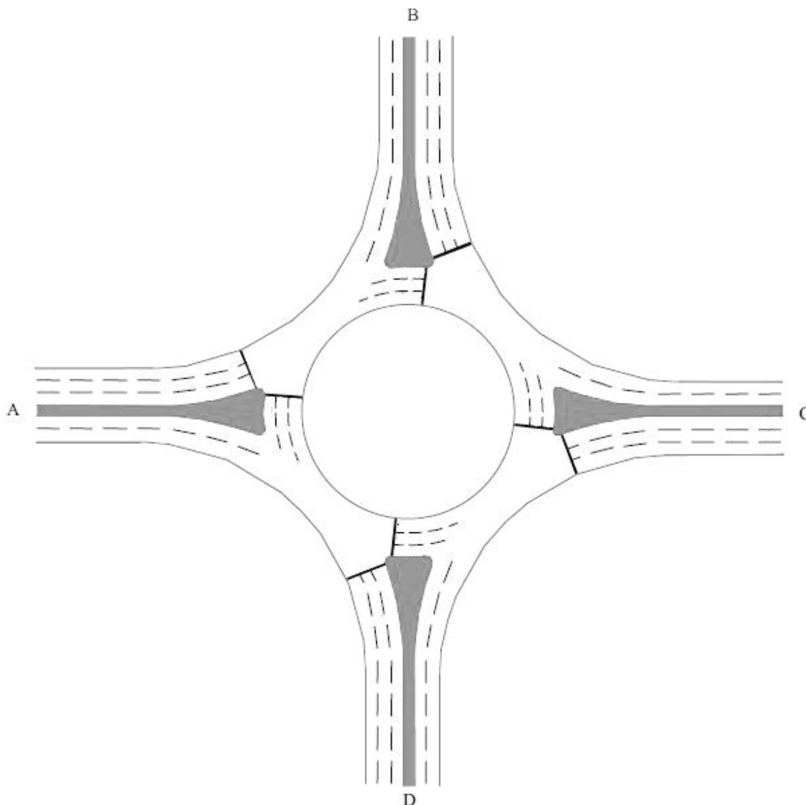
Figure 2.6 Illustrative layout of a signal-controlled roundabout
