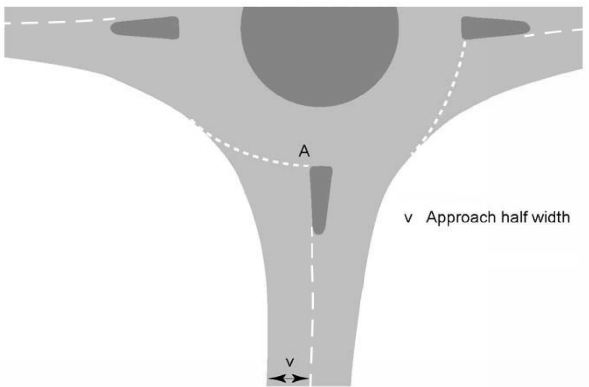
Figure 3.16 Entry width and approach half width
