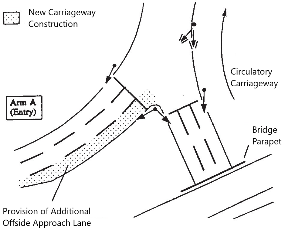
Figure 4.3.1N Provision of an additional offside approach lane
