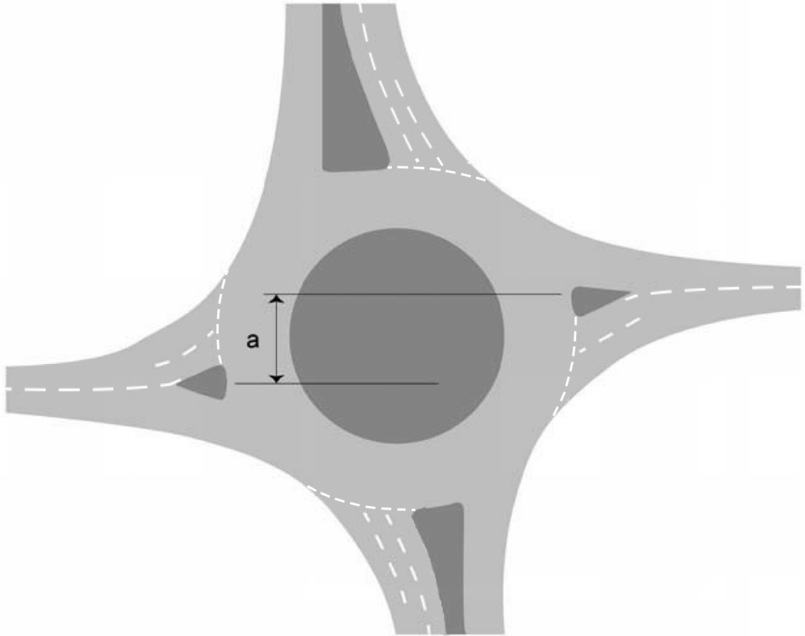
Figure 3.26.1 Staggering of east-west arms to increase deflection
