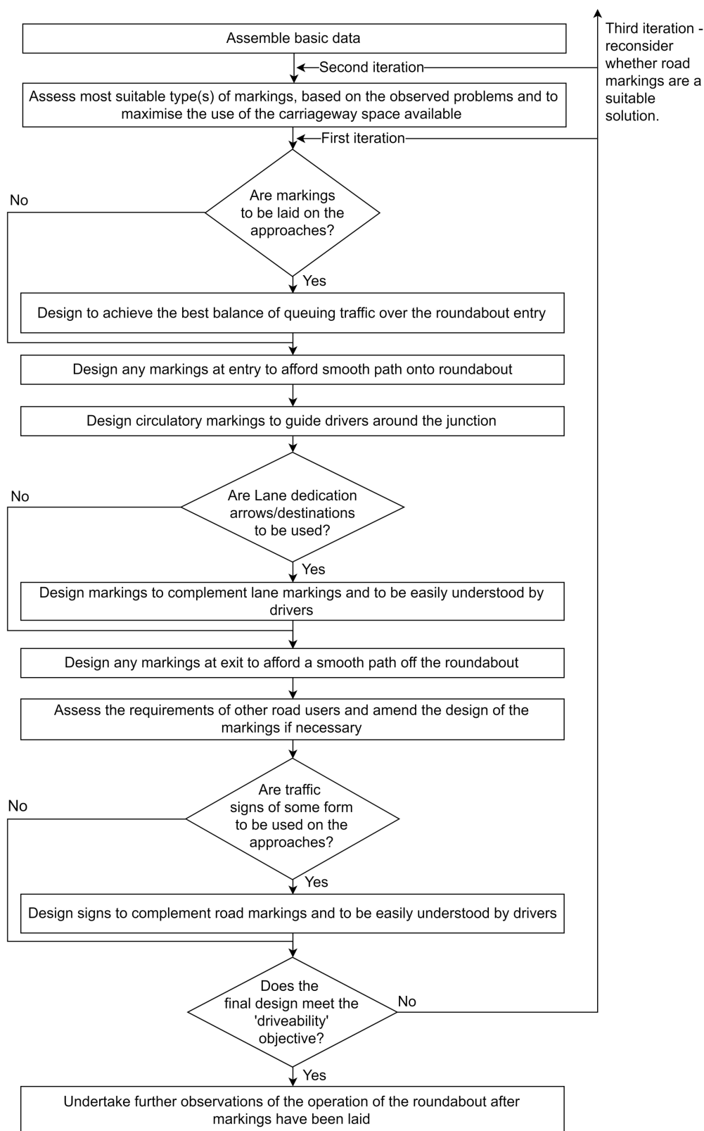
Figure D.2 Flow chart illustrating design principles
