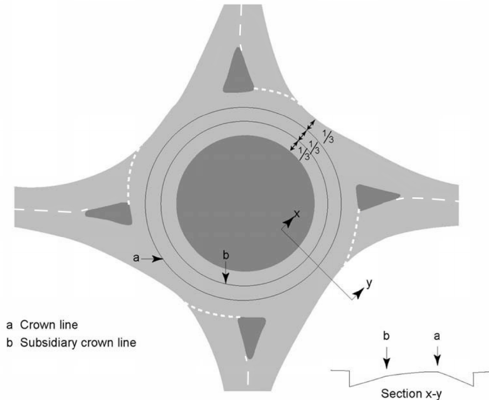
Figure 3.30.3N2 Using two crown lines
