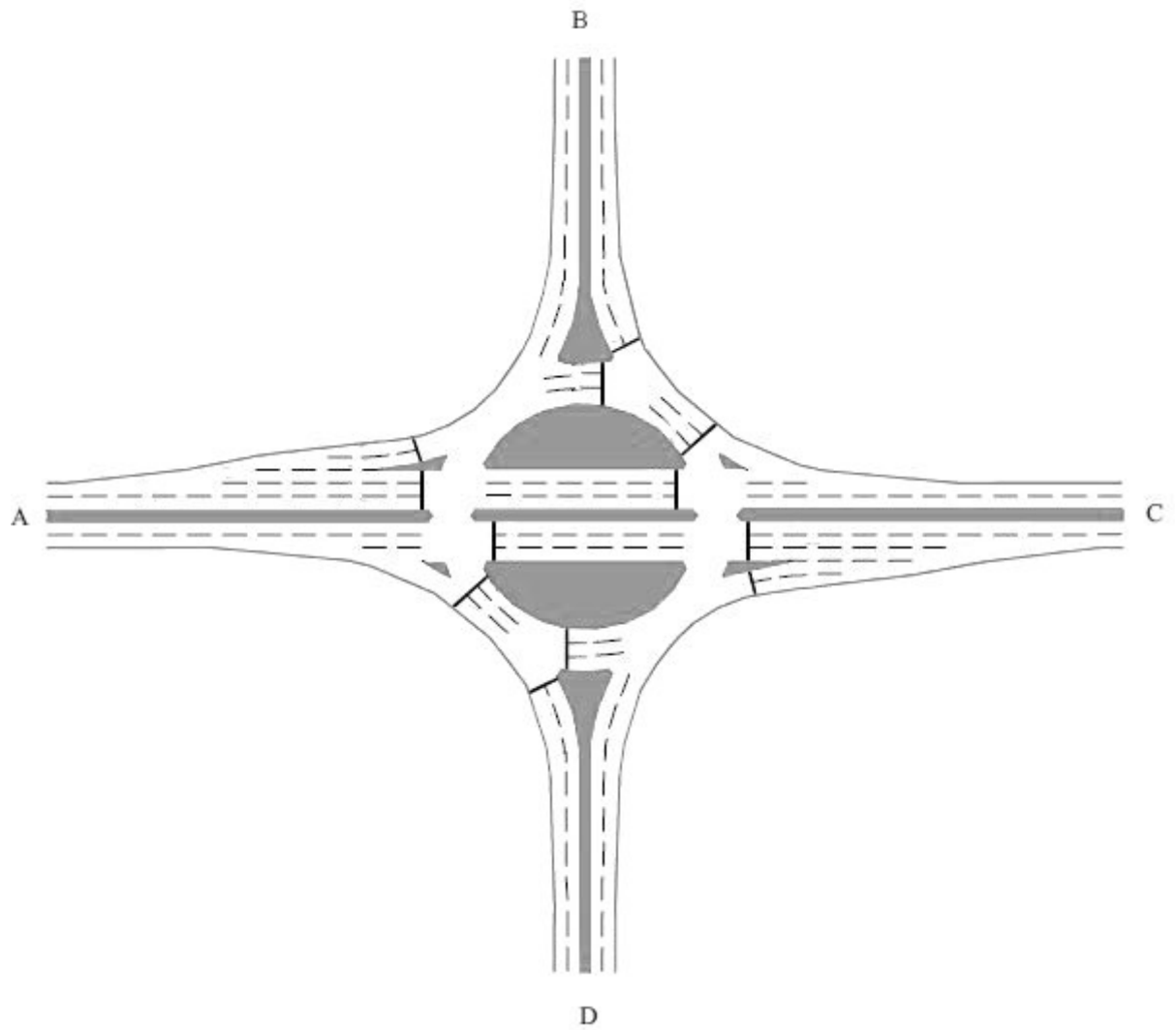
Figure 2.7a Illustrative layout of a through-about
