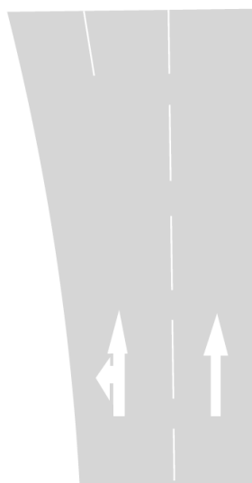
Figure 3.27.6a Example of approach markings
