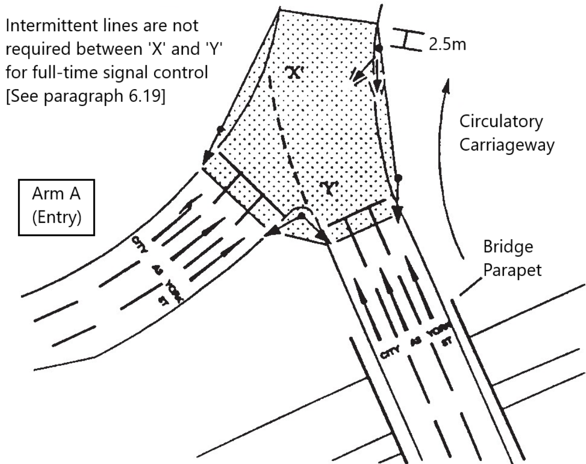
Figure 4.9.1 Junction intervisibility zone on a signal-controlled roundabout
