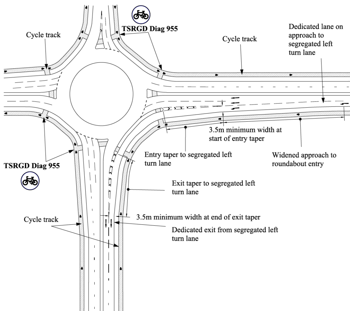
Figure 8.10N2b Dedicated approach and exit for SLTL including cycle track
