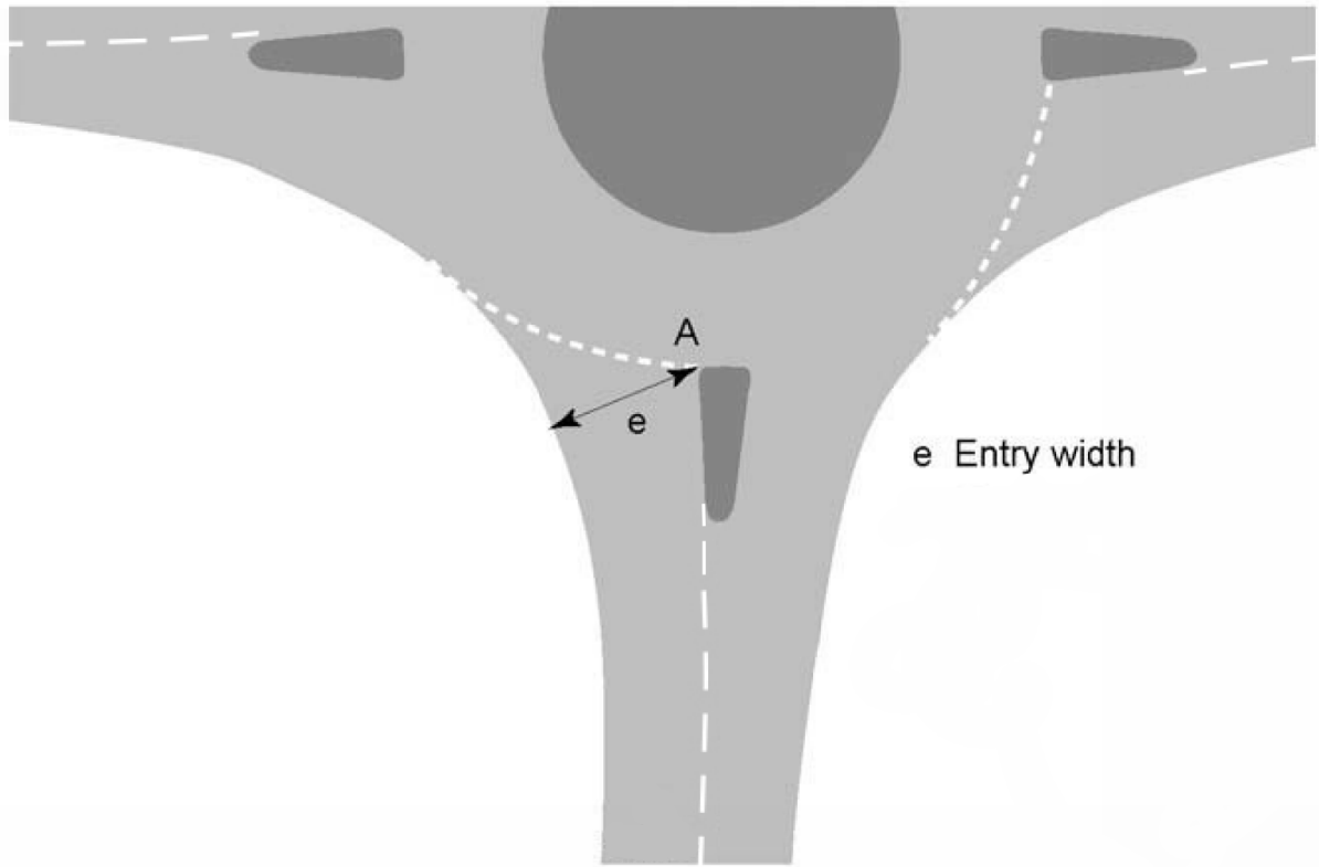
Figure 3.11 Entry width and approach half width
