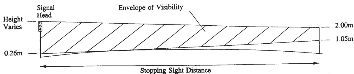
Figure 4.8 Visibility requirements to a signal head
