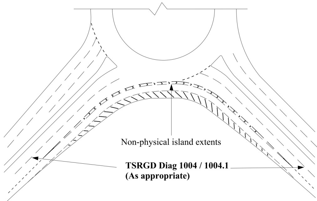
Figure 6.22 Generic non-physical SLTL
