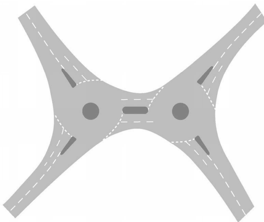
Figure 2.13 Illustrative layout of a double roundabout
