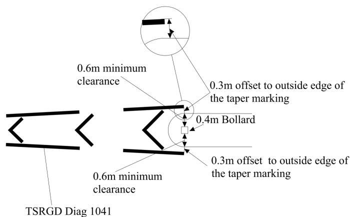
Figure 6.37.2 Termination of taper hatching at physical island
