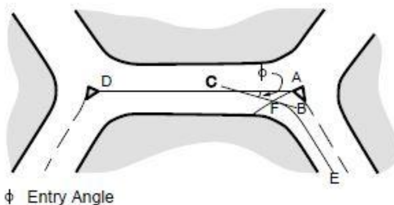
Figure B.1 Measurement of \phi where the distance circulatory carriageway between an entry and the next exit is approximately straight and more than about 30 metres
