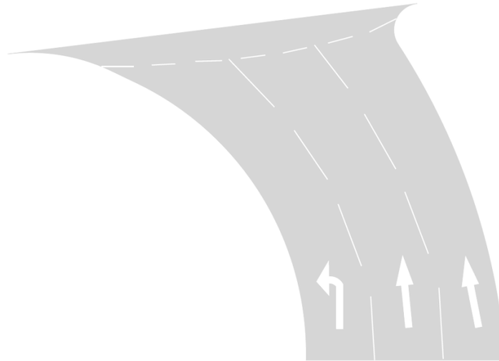
Figure 3.27.6b Example of entry markings
