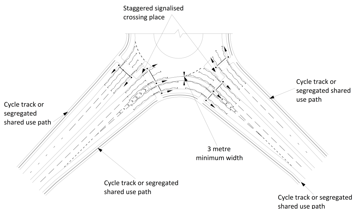
Figure 8.9 Cycle tracks and signal controlled crossing places at segregated left turn lane
