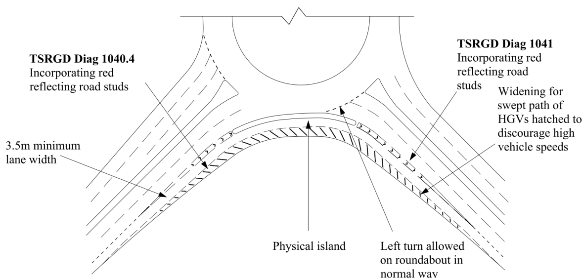
Figure 6.2.1 Generic physical SLTL
