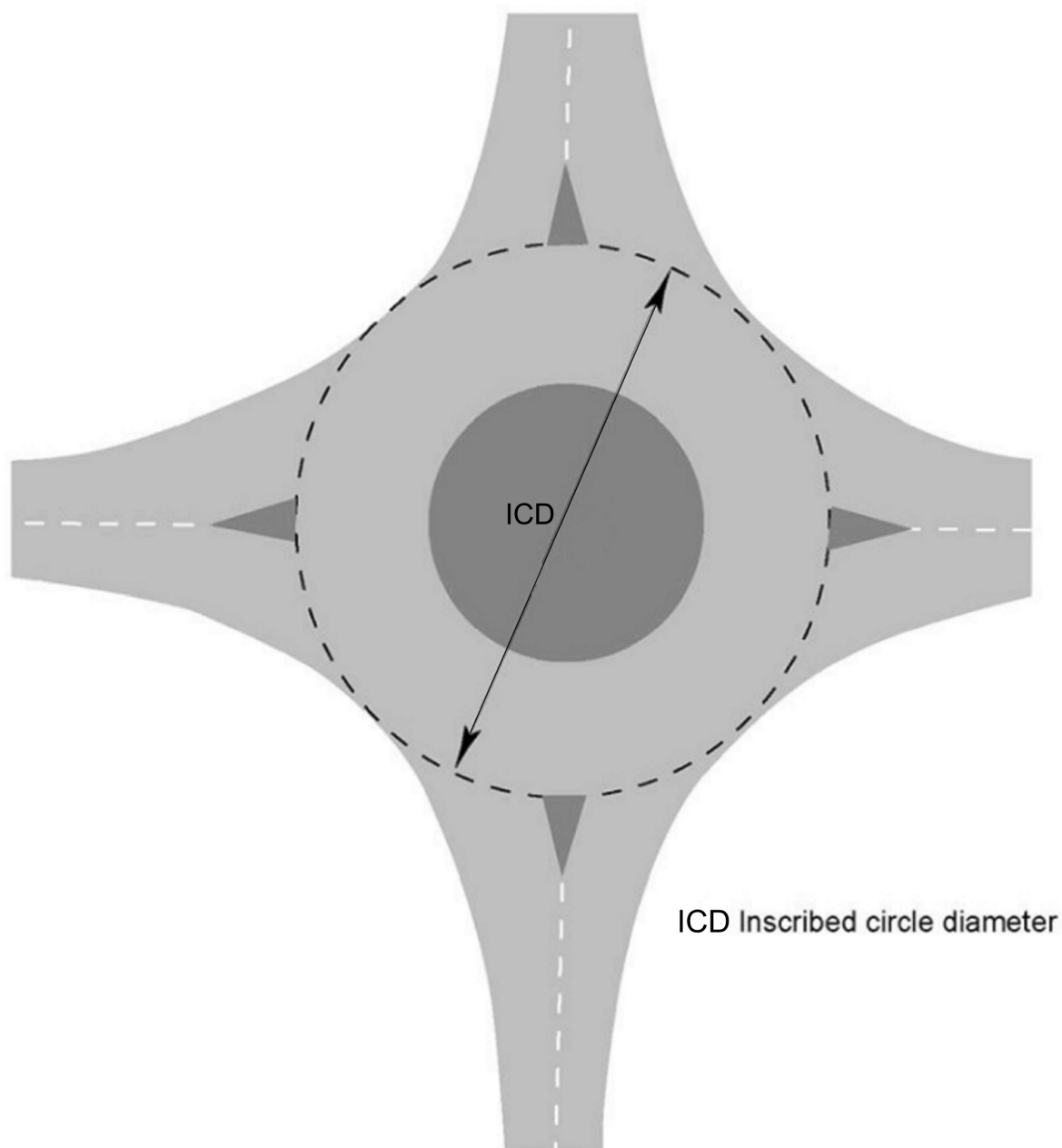
Figure 3.2 Inscribed circle diameter at a normal or compact roundabout
