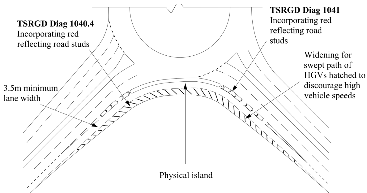
Figure 6.53.2b Generic physical segregated left turn lane
