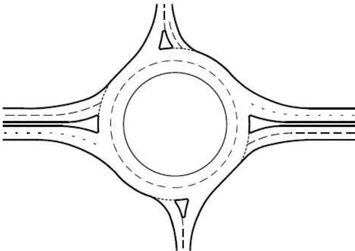
Figure D.3 Concentric markings
