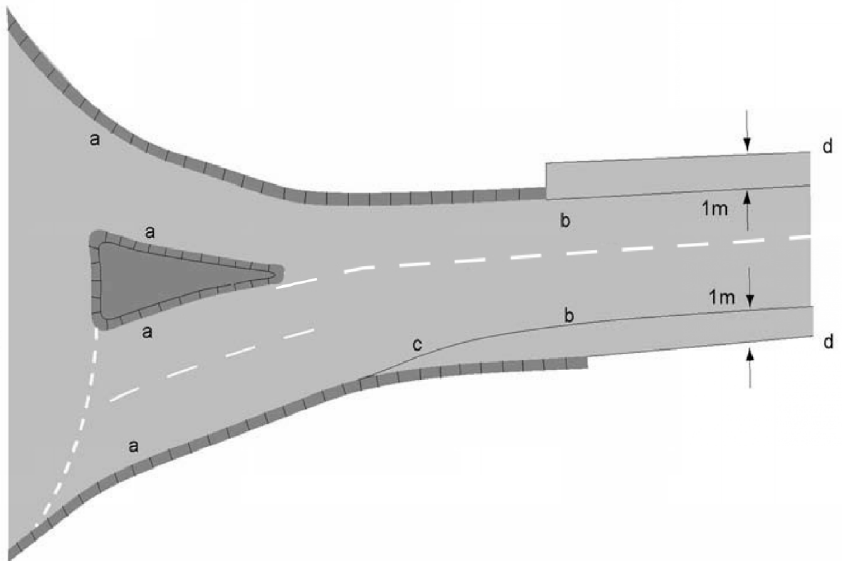
Figure 3.54Na Method of terminating edge strips on a single carriageway approach to a roundabout
