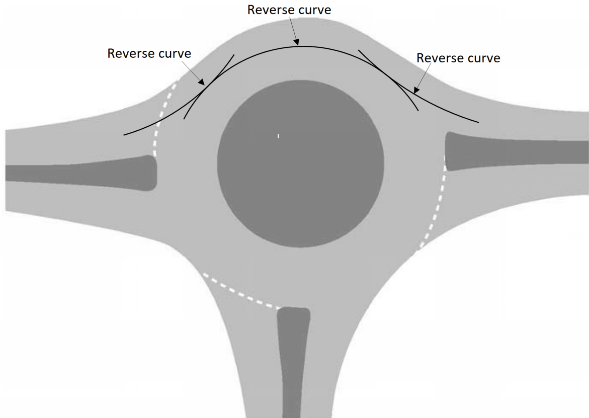
Figure 3.6.9N2 Three-arm roundabout illustrating reverse curvature
