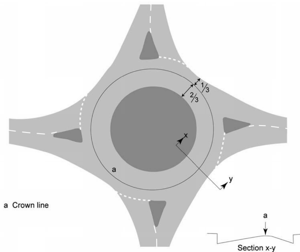
Figure 3.30.3N1b Using one crown line to divide the carriageway into the ratio 2:1
