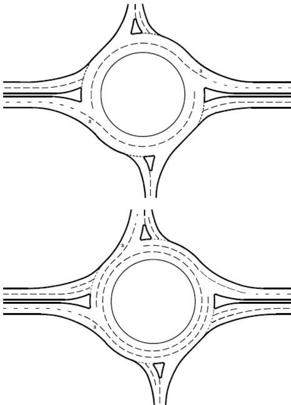
Figure D.5 Concentric spiral markings
