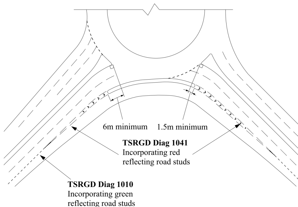
Figure 6.20 Physical SLTL without crossings
