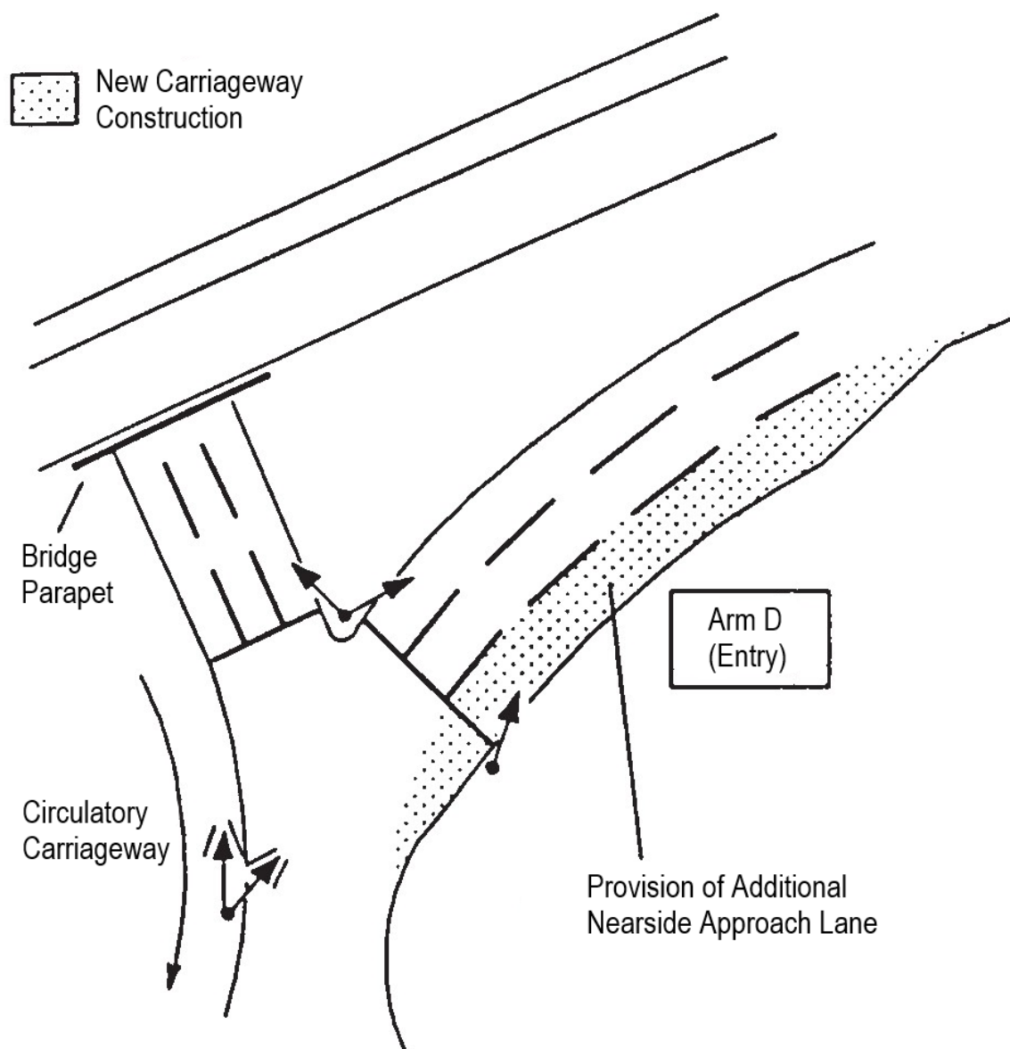
Figure 4.3.2N Provision of an additional nearside approach lane
