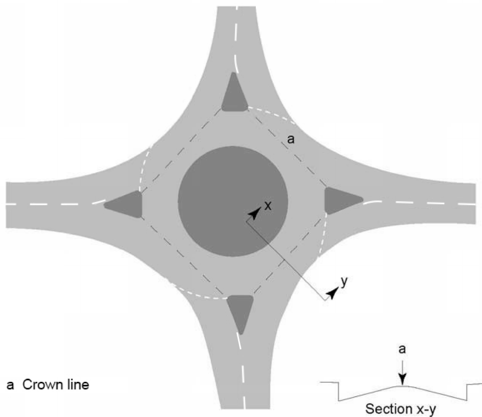
Figure 3.30.3N1a Using one crown line to join traffic islands
