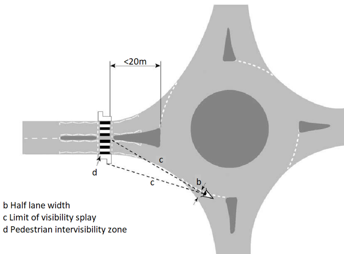
Figure 3.53 Visibility measured at entry to pedestrian crossing at next exit
