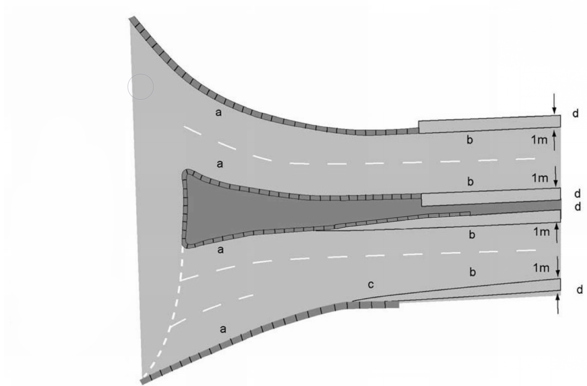
Figure 3.54Nb Method of terminating edge strips on a dual carriageway approach to a roundabout
