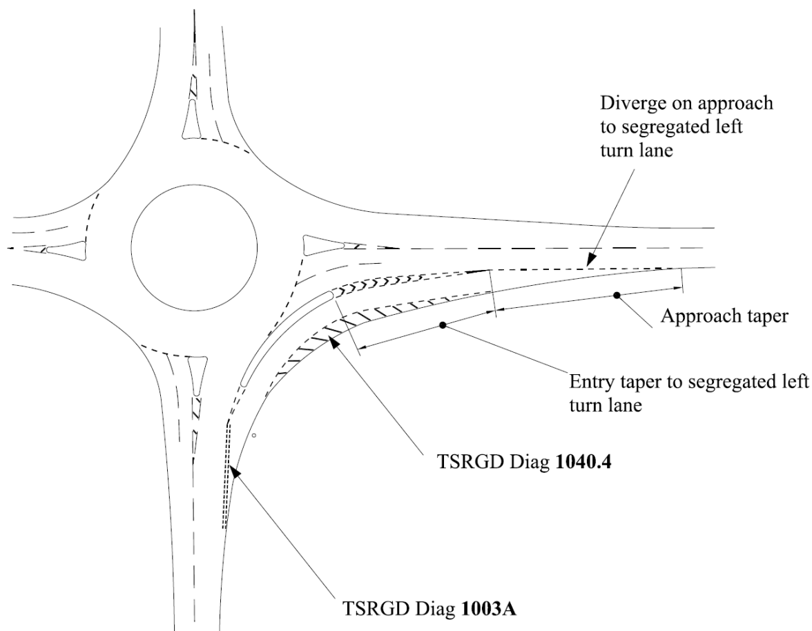
Figure 6.31 Physical SLTL approach taper
