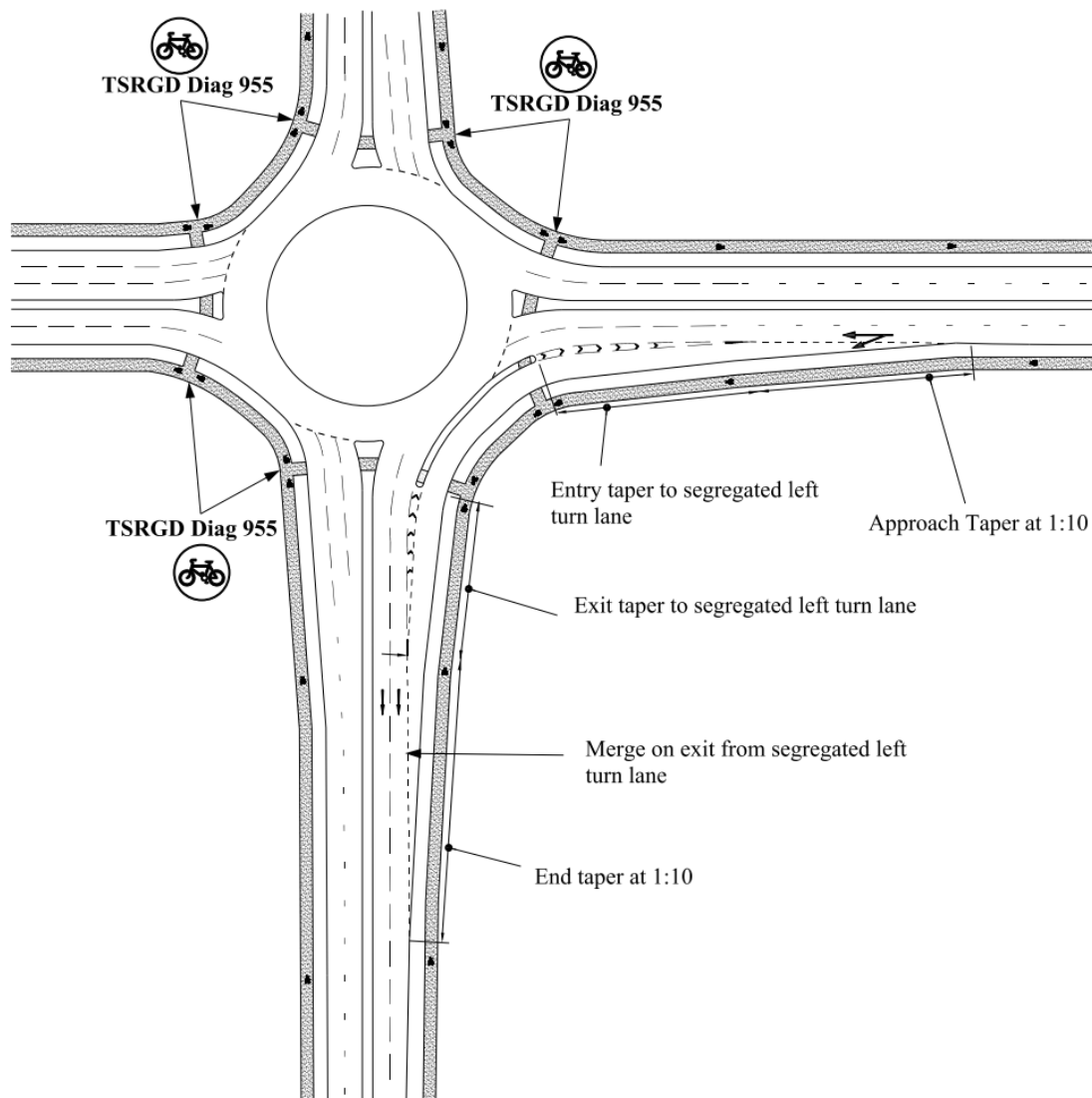
Figure 8.10N2a Diverge/merge layout SLTL island, 50 metres in length including cycle track
