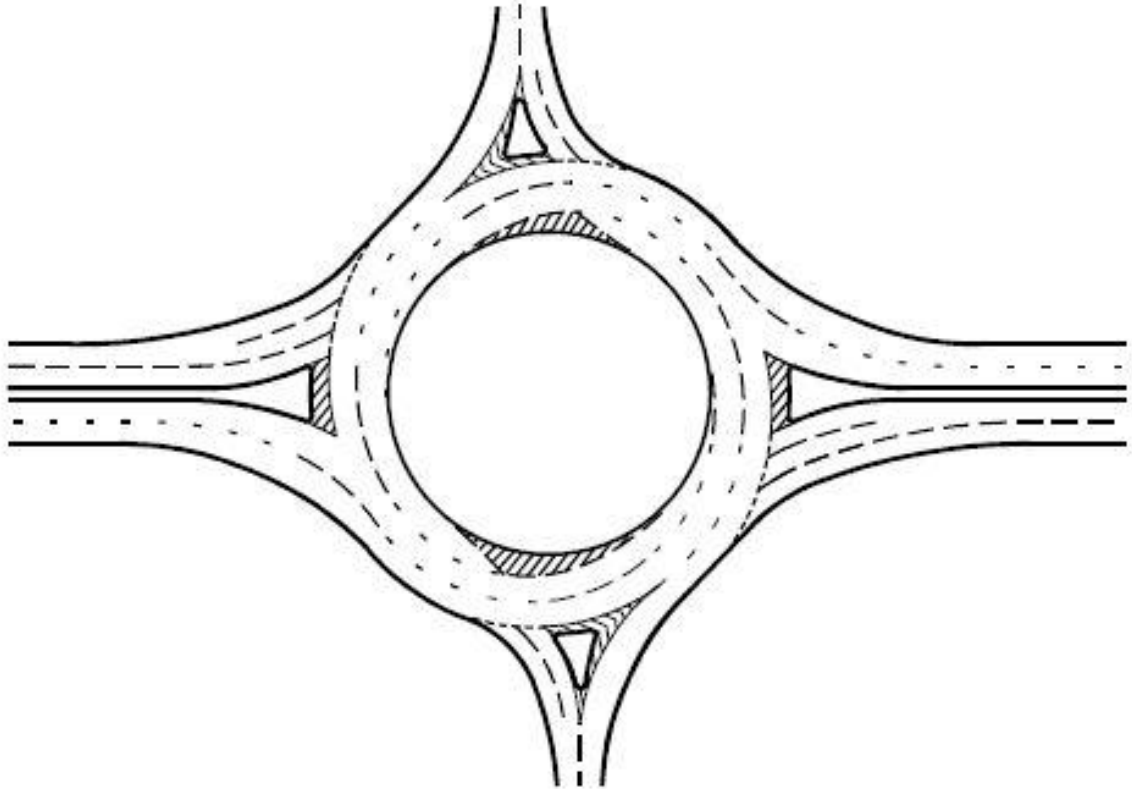
Figure D.7 Use of different lane line types within a spiral markings system
