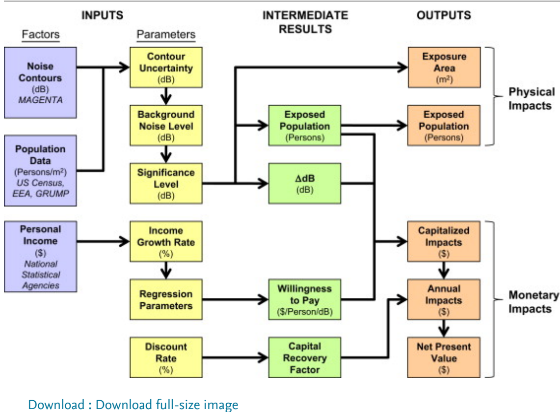
Fig. 4. Schematic of income-based noise monetization model.
