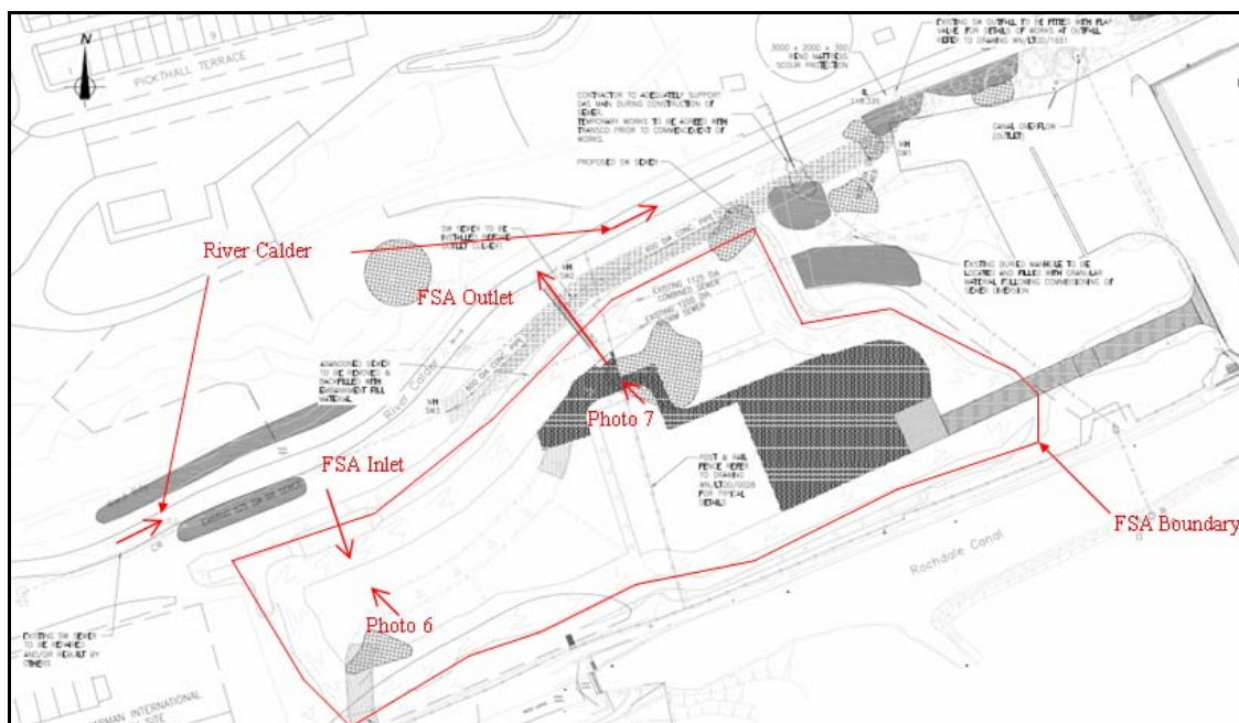
Figure 2.3: Millwood FSA – Non-impounding
