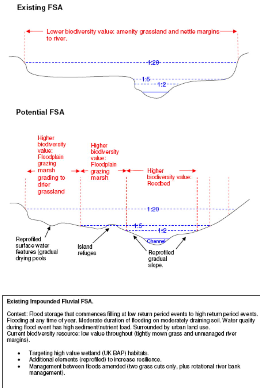
Figure 6.3(a). Existing impounded FSAs
