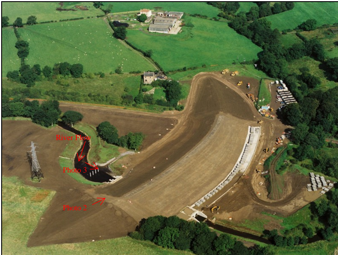
Photo 1: River Gaunless – Impounding FSA (at end of construction)
