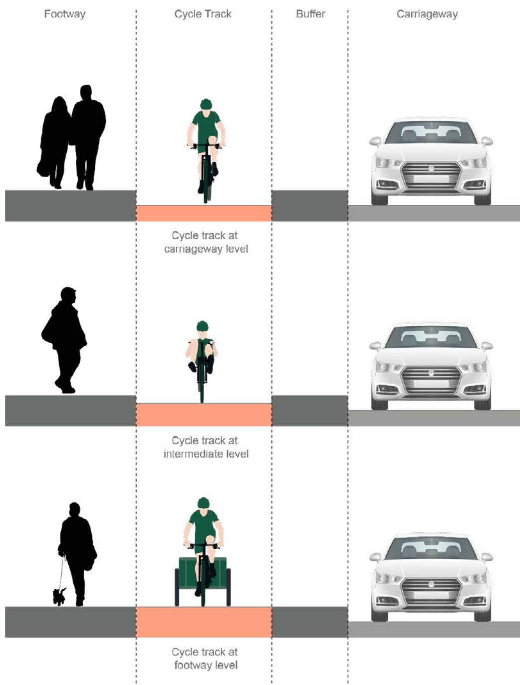
Figure 6.3: Cycle tracks with full kerb separation from carriageway
