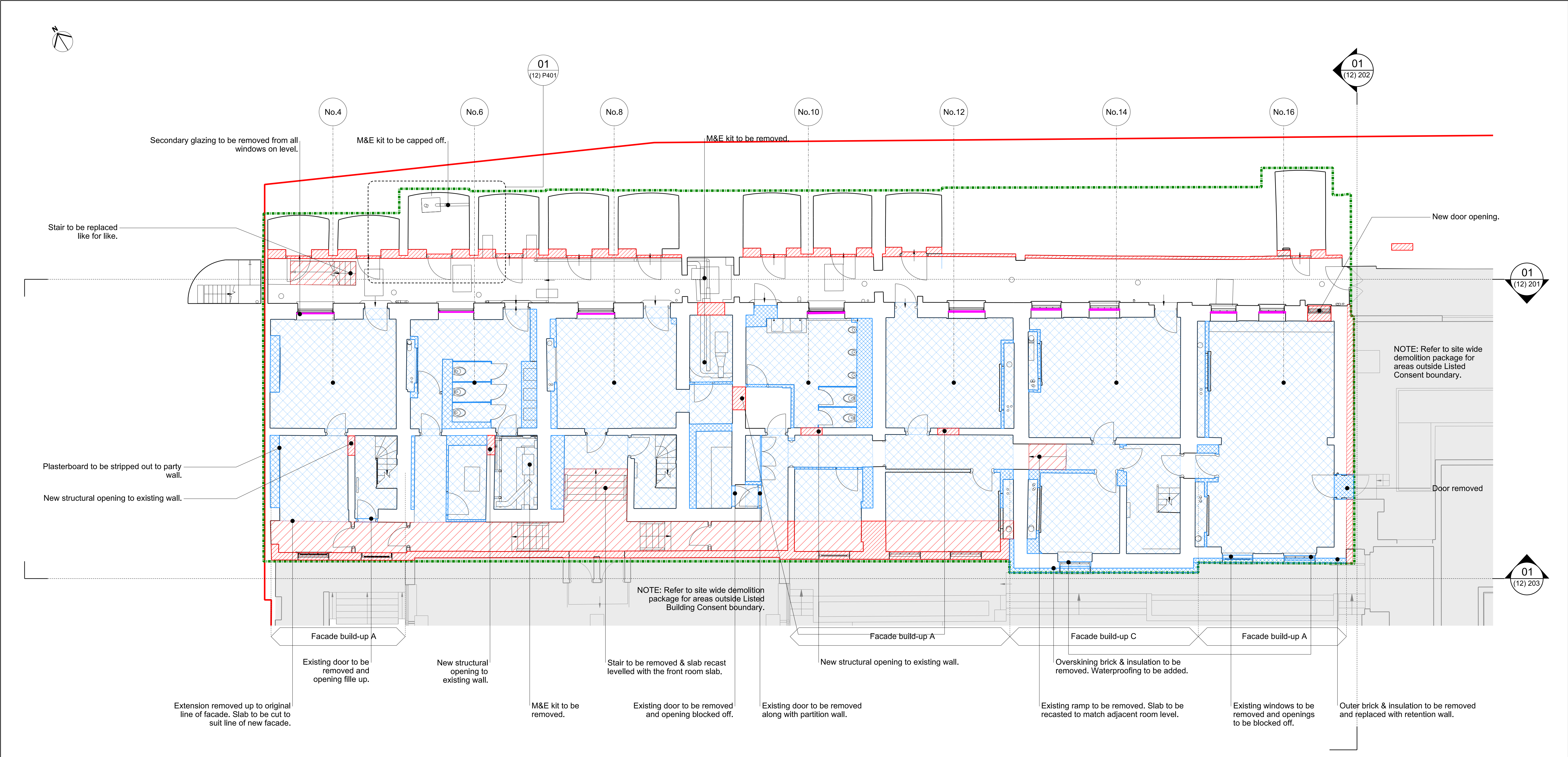
01 LOWER GROUND FLOOR DEMOLITION PLAN
