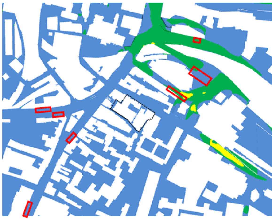
Configuration 1: Summer Wind Comfort (Ground Level)
