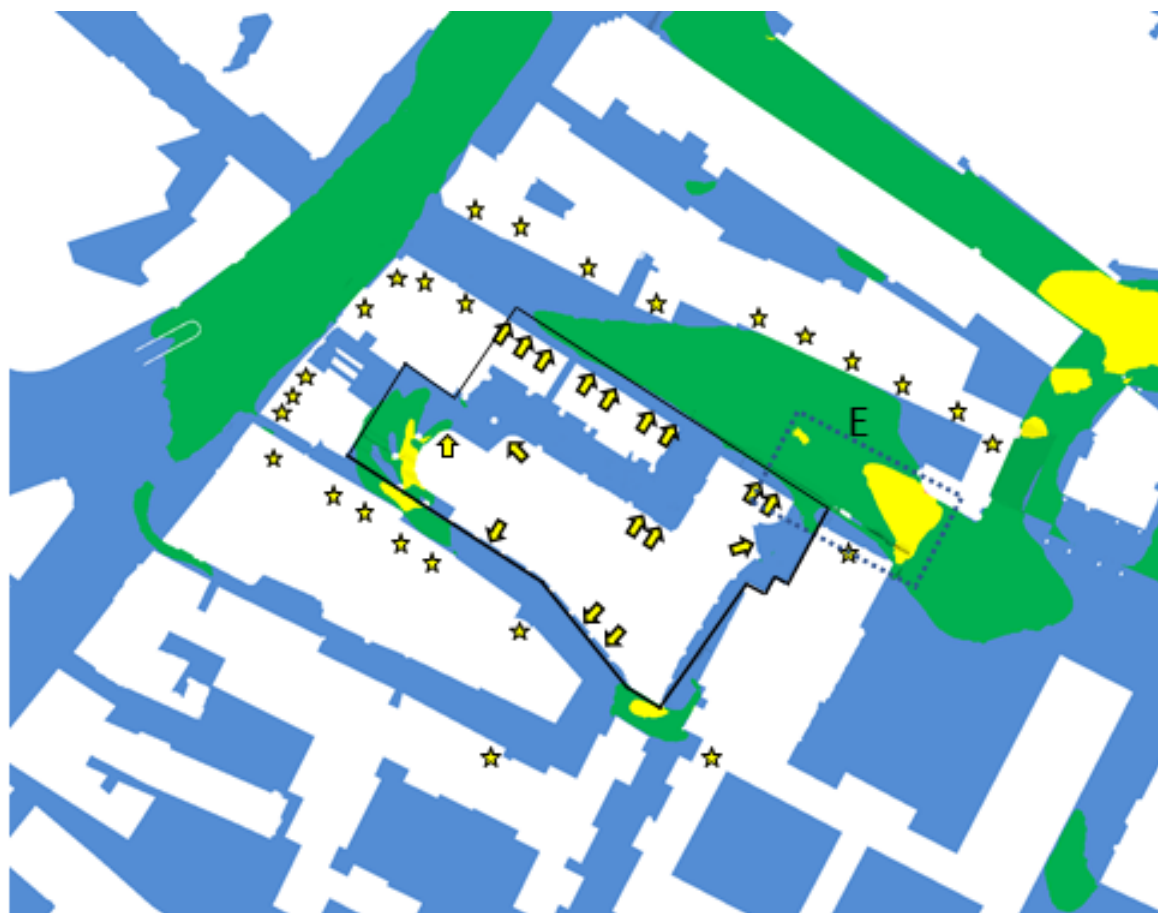
Configuration 2: Winter Wind Comfort (Ground Level)
