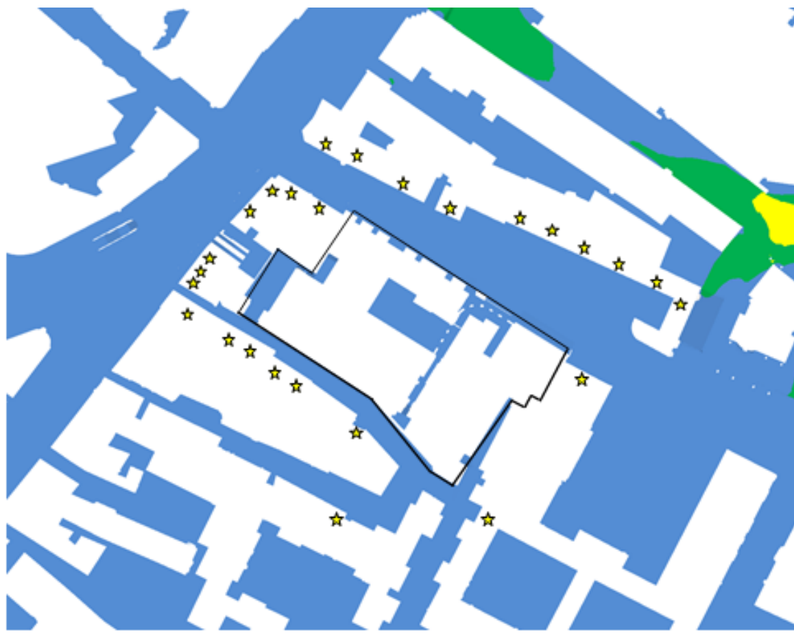
Configuration 1: Summer Wind Comfort (Ground Level)
