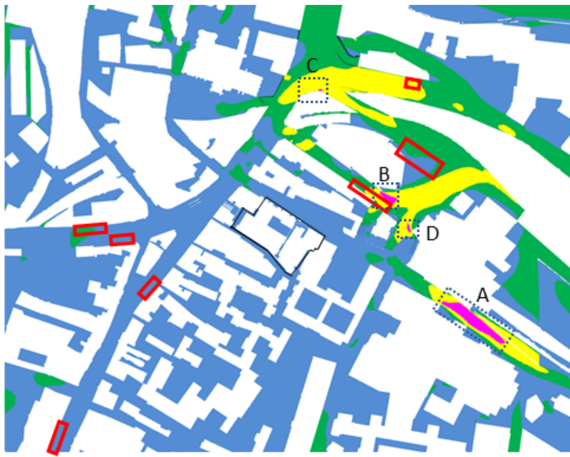
Configuration 1: Winter Wind Comfort (Ground Level)
