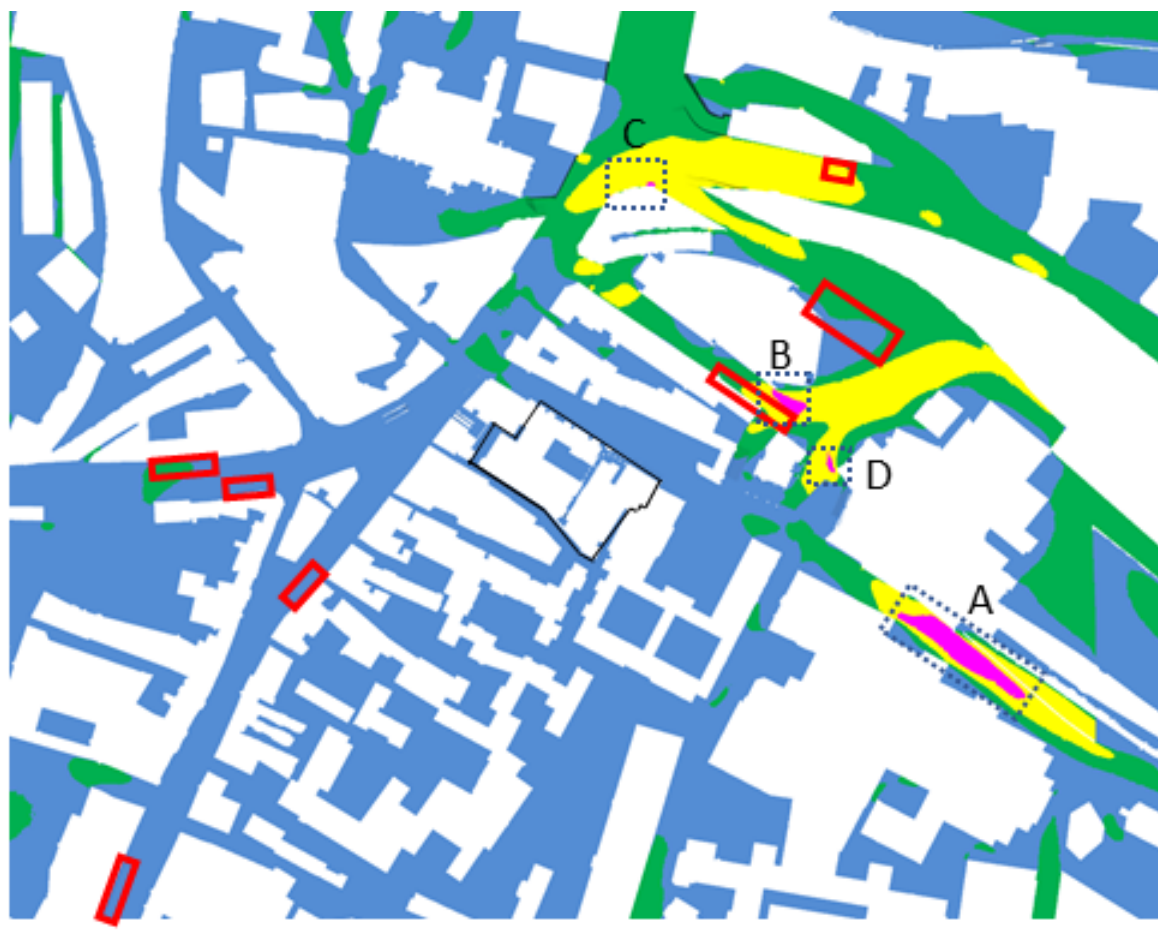
Configuration 1: Winter Wind Comfort (Ground Level)
