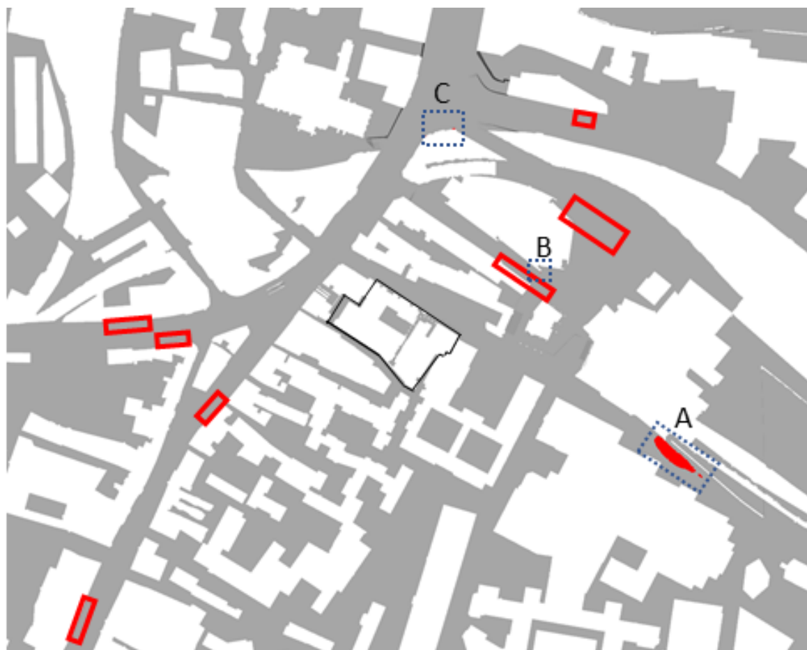
Configuration 1: Annual Wind Safety (Ground Level)
