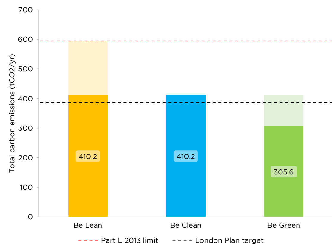
Figure 4-1 Regulated CO 2 emissions at each stage of the energy hierarchy for the whole Proposed Development using SAP 10.0 carbon factors
