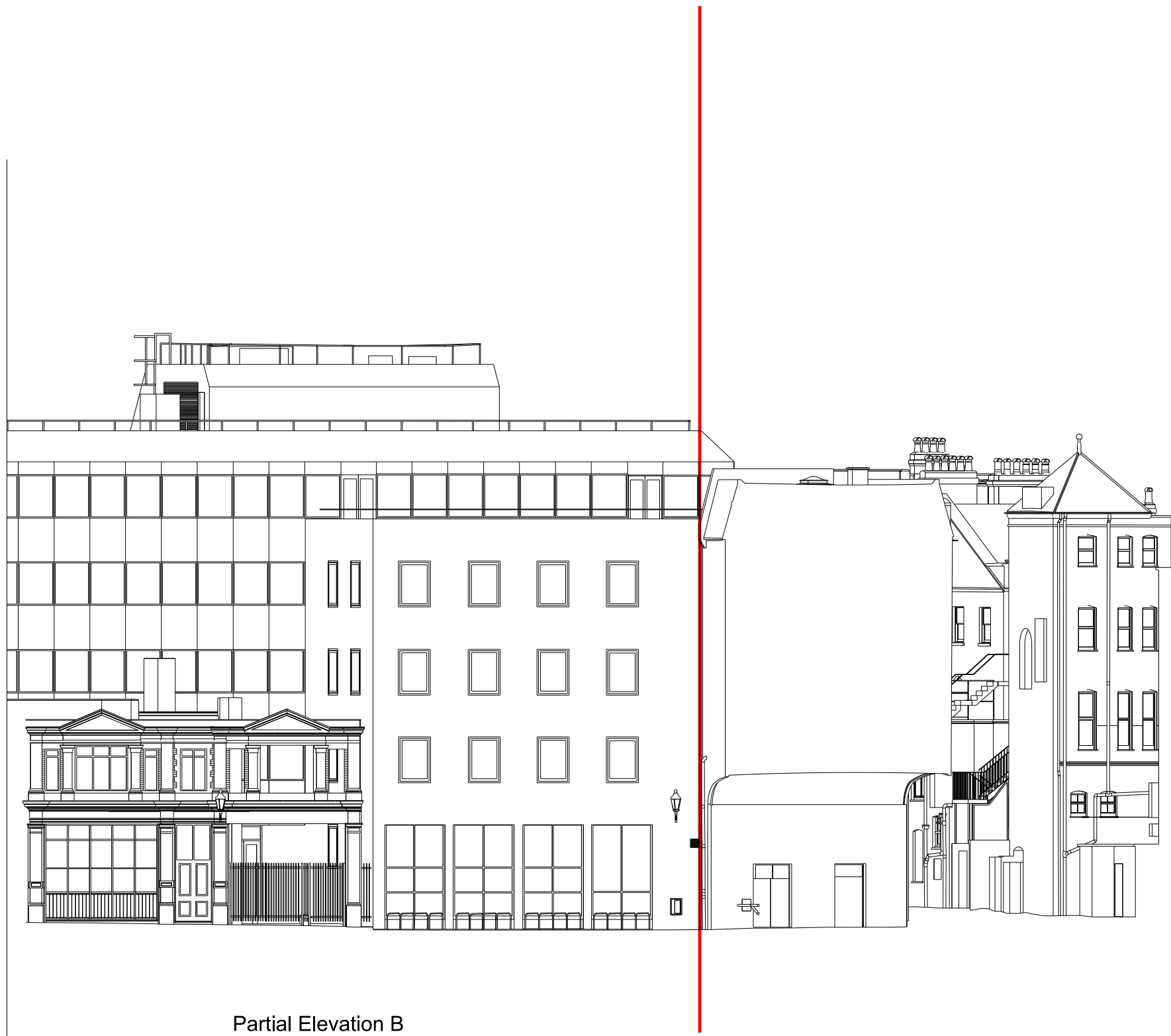
Partial Elevation B
