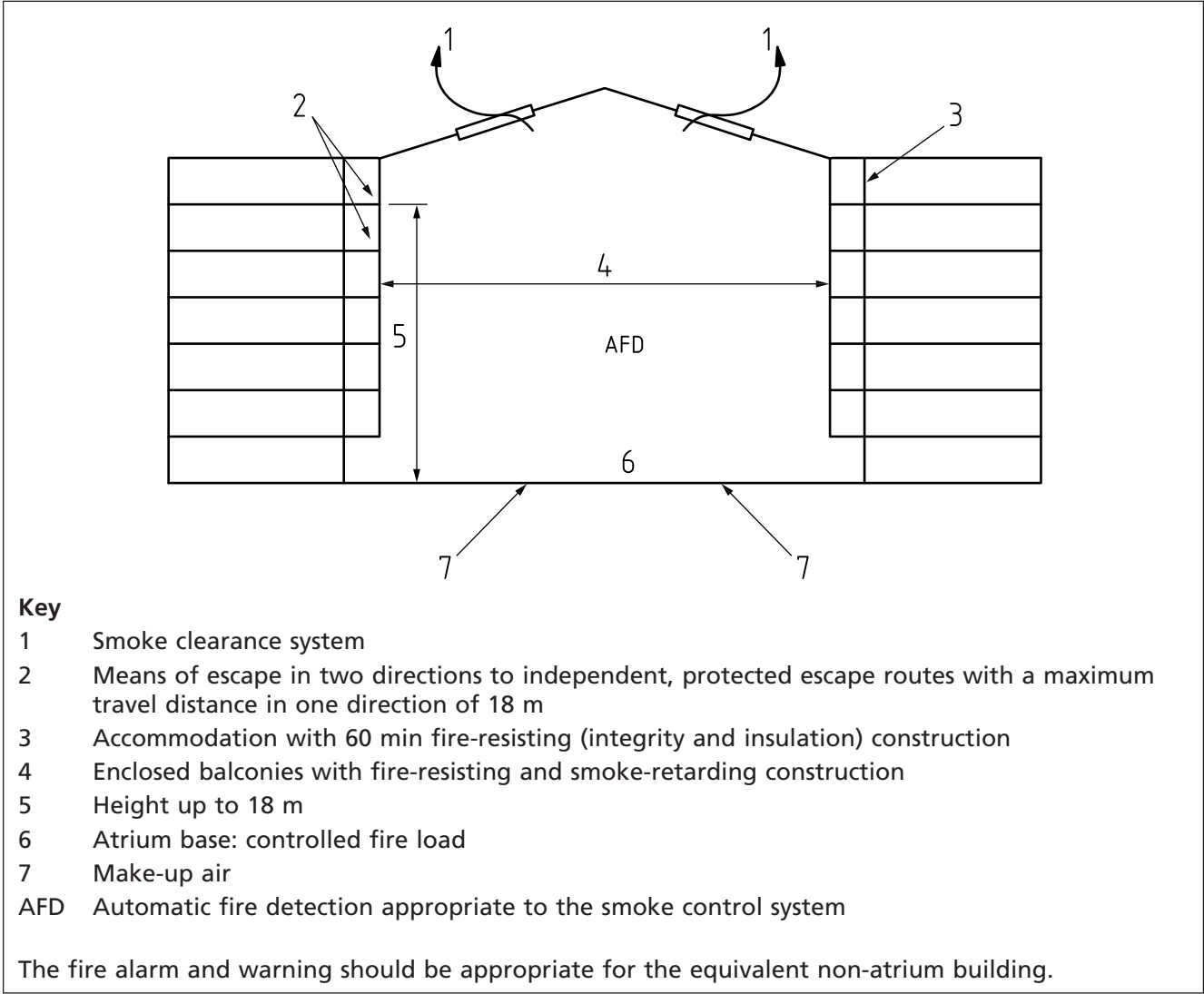
Figure C.5 Exemplar 3b: Atrium base: controlled fire load
