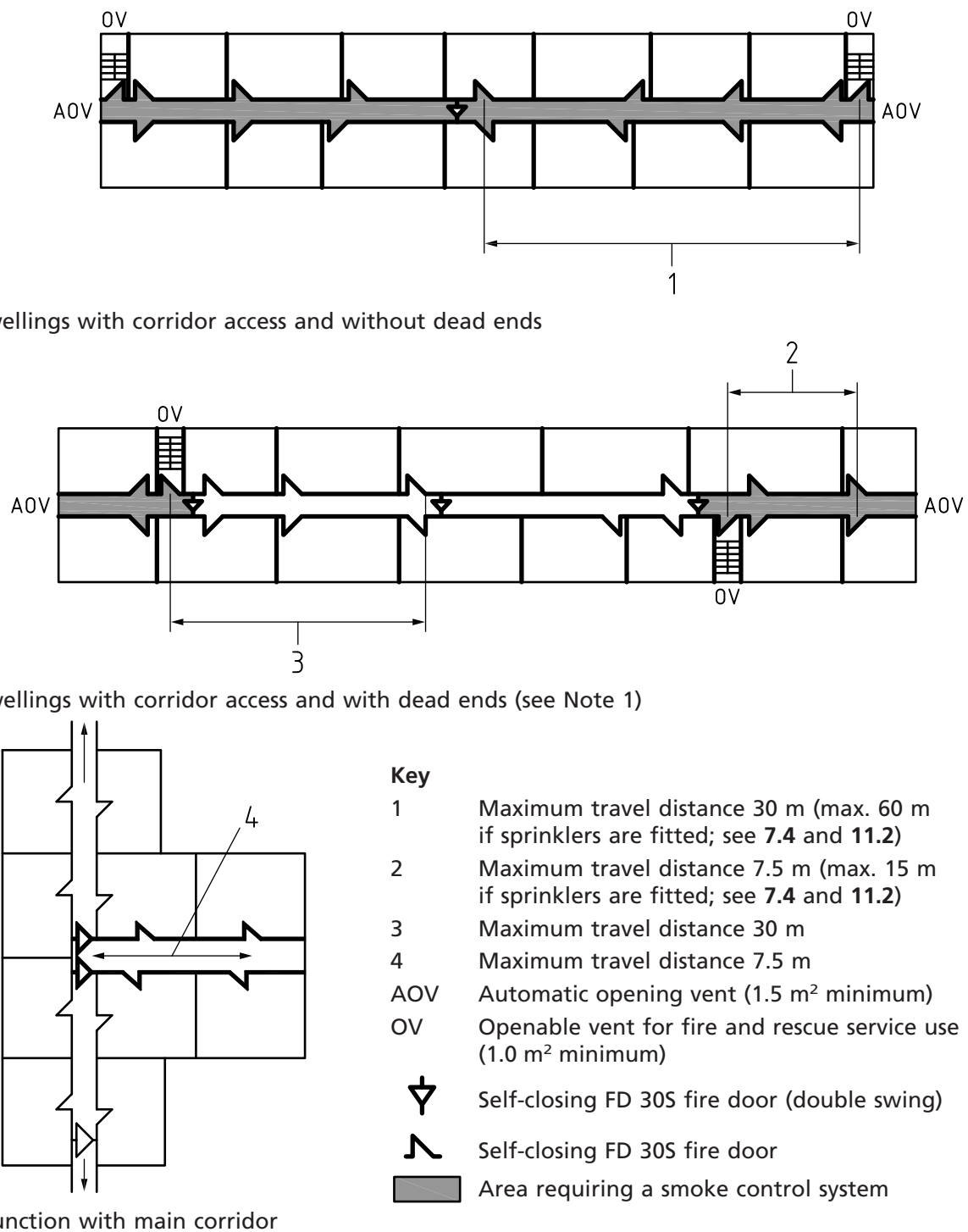
Figure 7 Common escape routes in multi stair buildings
