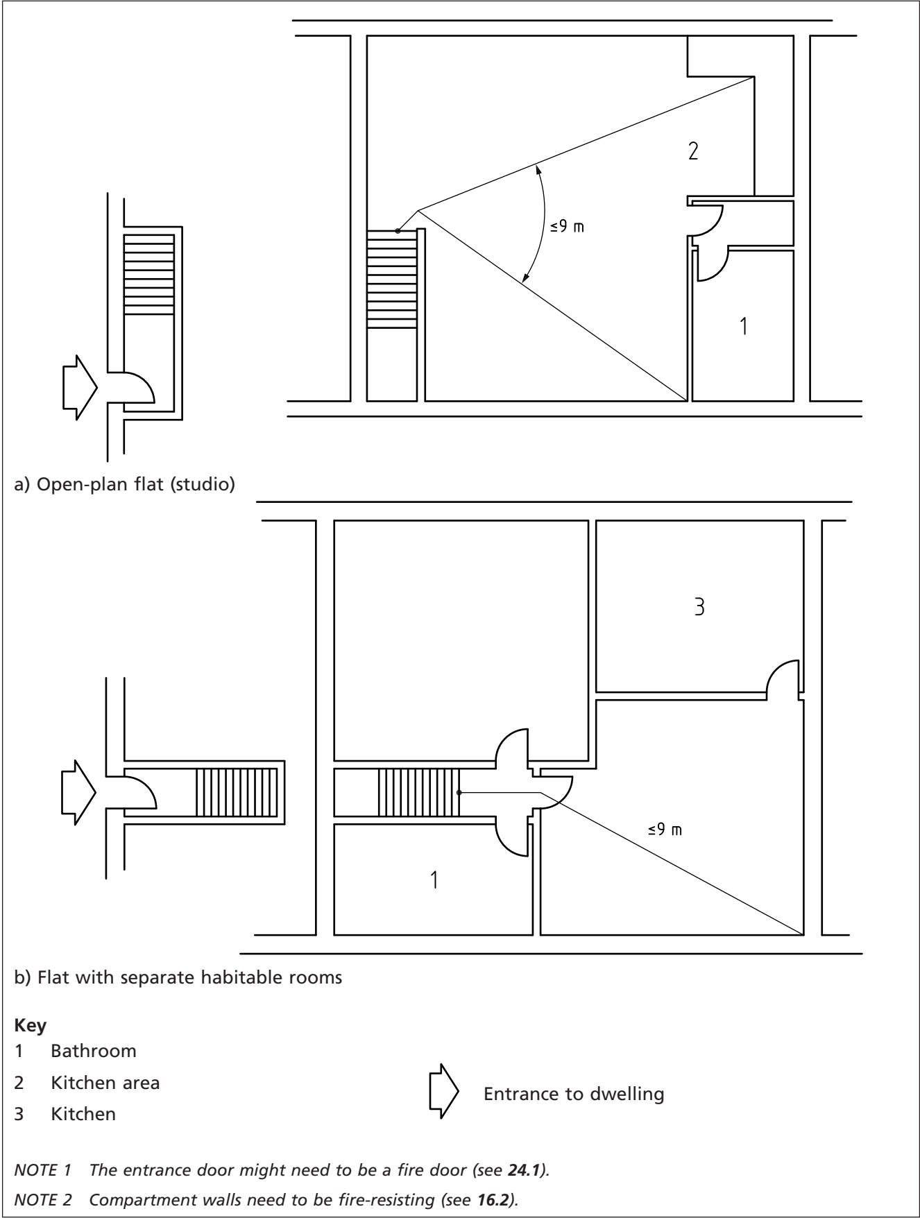
Figure 13 Flat (entered from below) with a restricted travel distance
