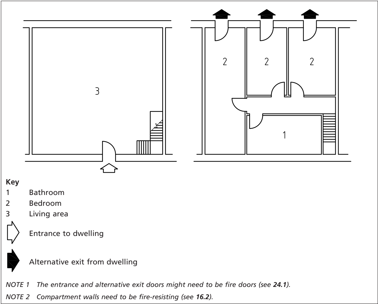
Figure 4 Open-plan maisonette
