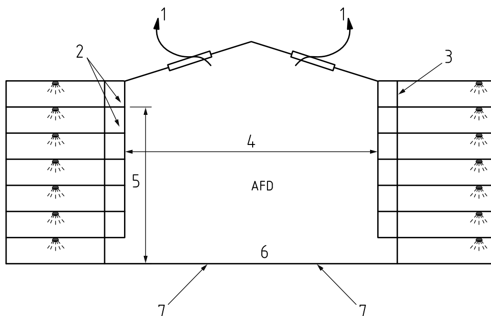
Figure C.6 Exemplar 3c: Atrium base: controlled fire load
