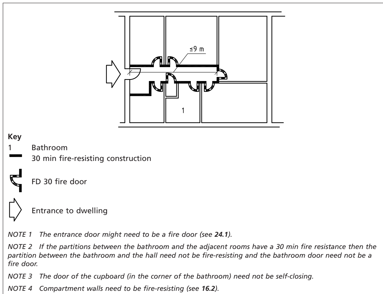
Figure 11 Flat with a protected entrance hall and restricted travel distance
