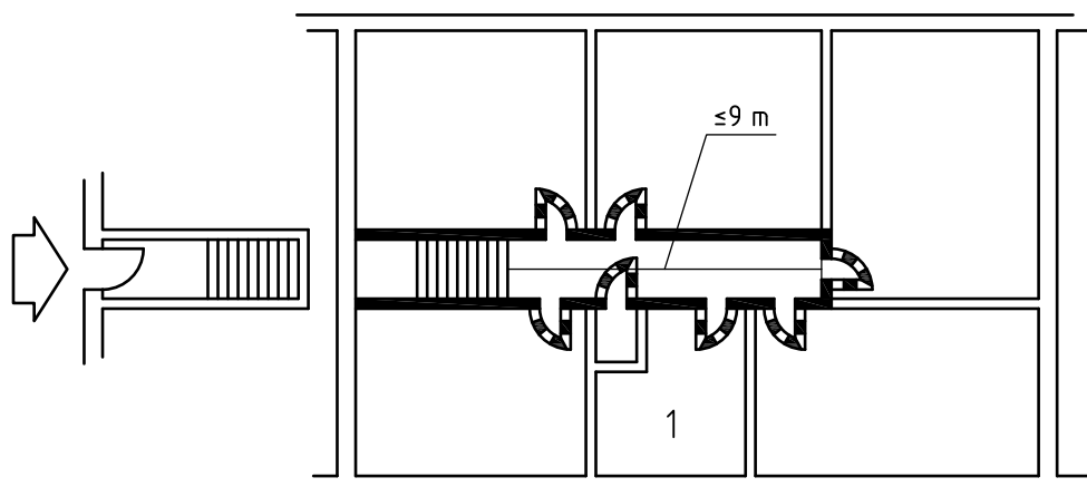
Figure 14 Flat (entered from below) with a protected entrance hall and restricted travel distance
