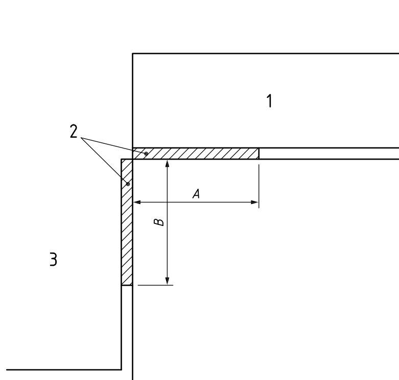
Figure 31 Protected routes forming an internal angle
