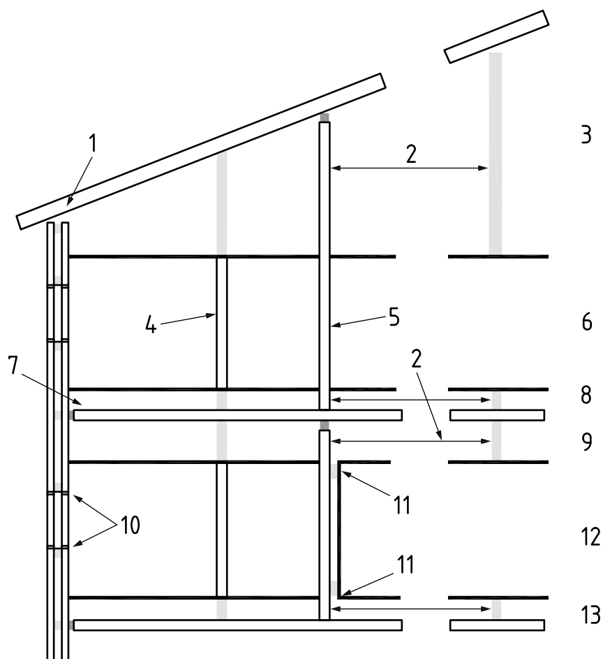
Figure 24 Provisions for cavity barriers
