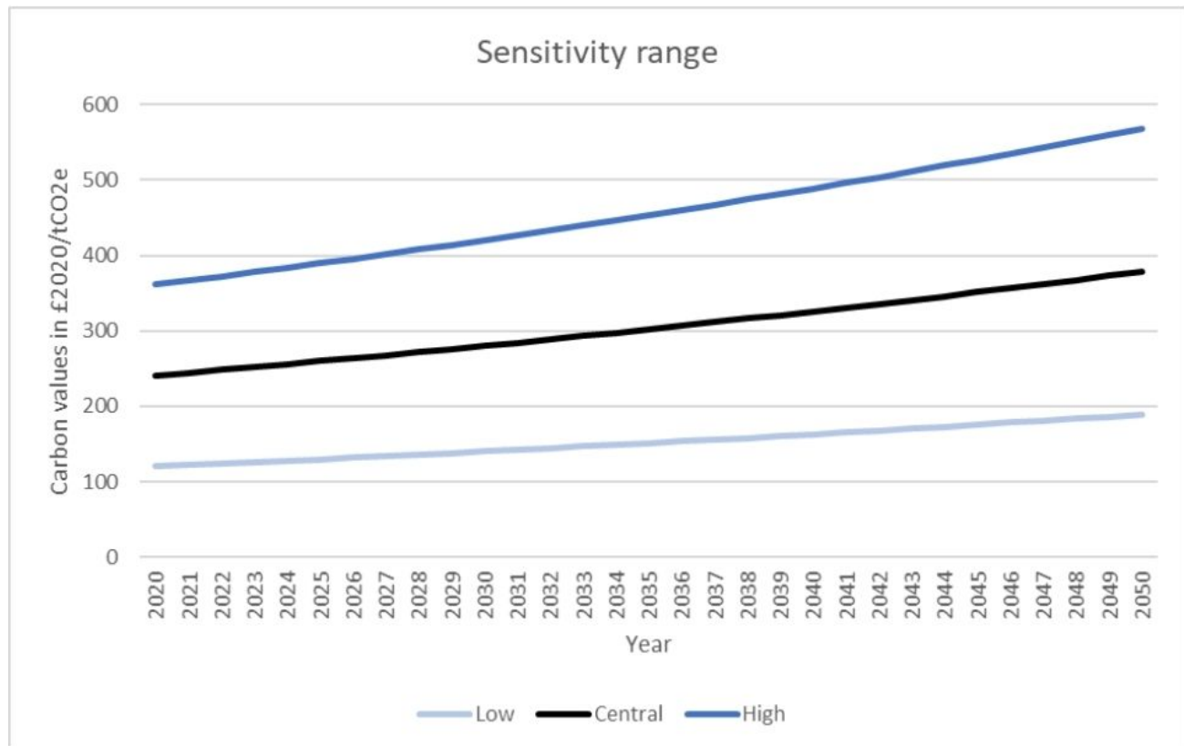
Figure 3: Sensitivity range of the updated carbon values.
