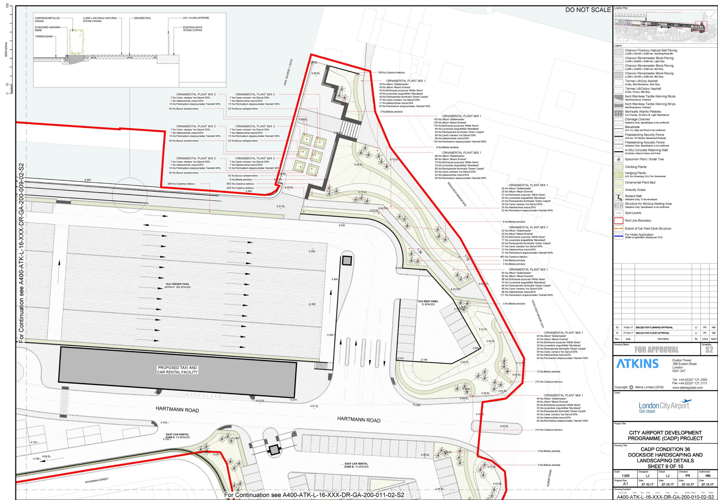
Figure 4.0.18: Dockside Hardscaping & Landscaping Details – Sheet 9 of 10 for approval
