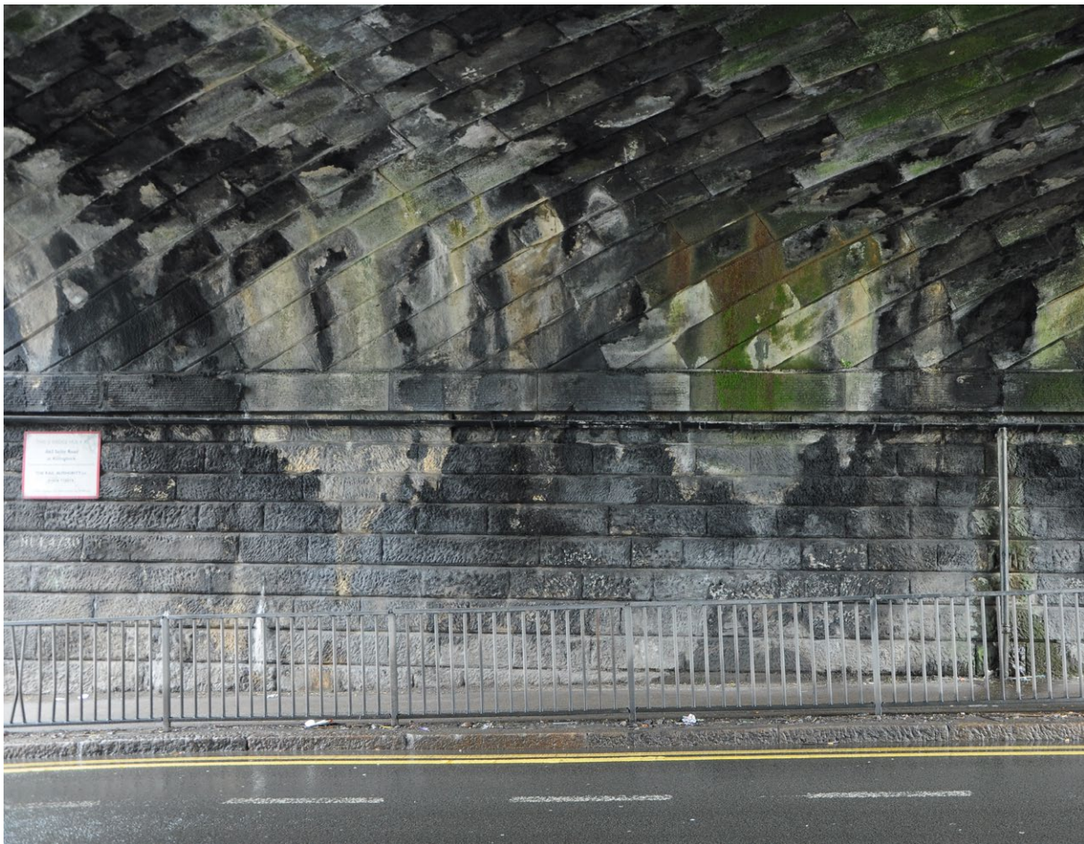
Examples of the outstanding stonework of Leeds & Selby Railway bridges, which were completed in 1834: above, Halton Dial (HUL4/30); opposite top, Roman Ridge Road (HUL4/14); opposite below, Austhorpe Lane (HUL4/21)
