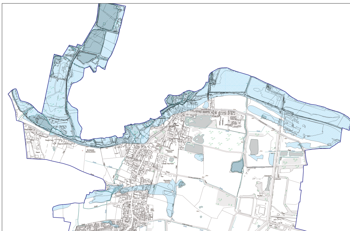
Figure 7.3 Historic Recorded Flood Areas
